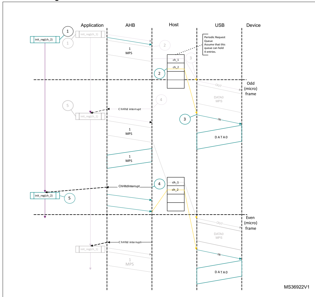
Figure 424. Normal isochronous IN transactions - DMA mode
