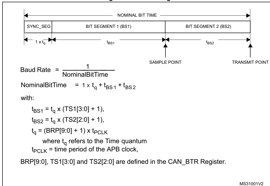
Figure 395. Bit timing
