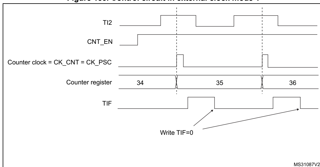
Figure 133. Control circuit in external clock mode 1
