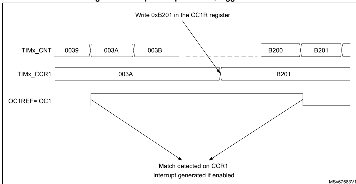
Figure 221. Output compare mode, toggle on OC1.
