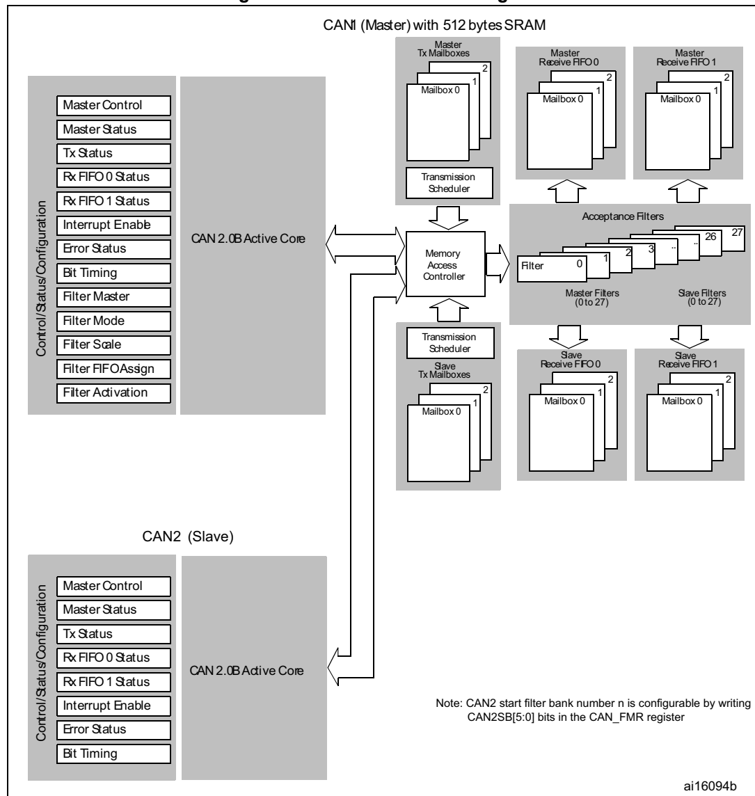
Figure 384. Dual-CAN block diagram
